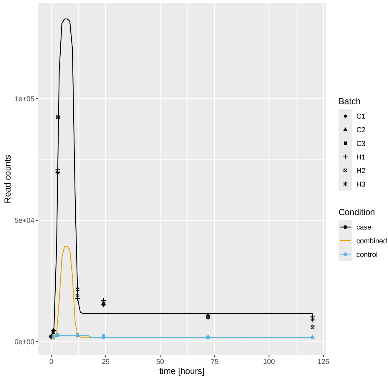
Pocillopora_acuta_Hlv2___TS.g28751.t1: log10 q = -74.9
