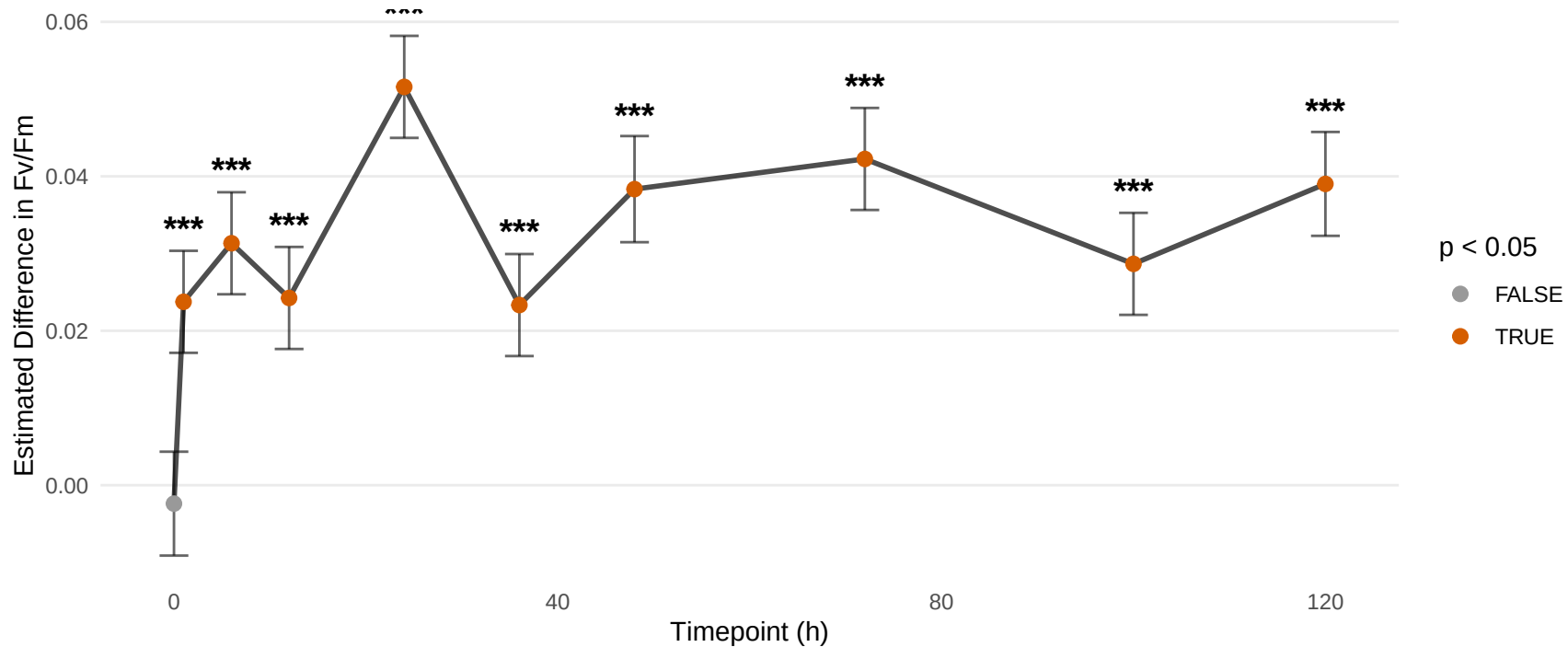
Estimated Treatment Effect (Control-Heat) on Fv/Fm
