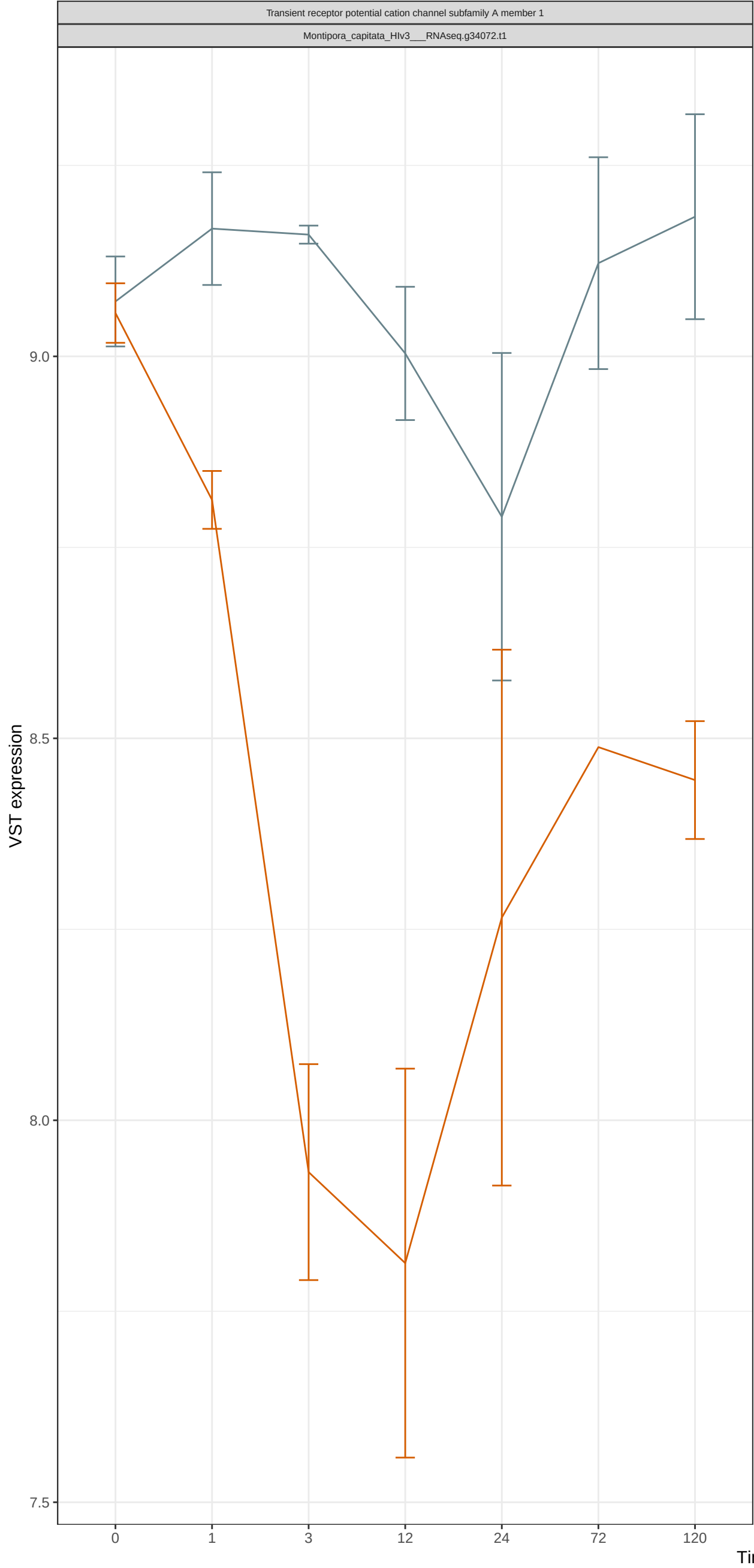
Cluster 1
