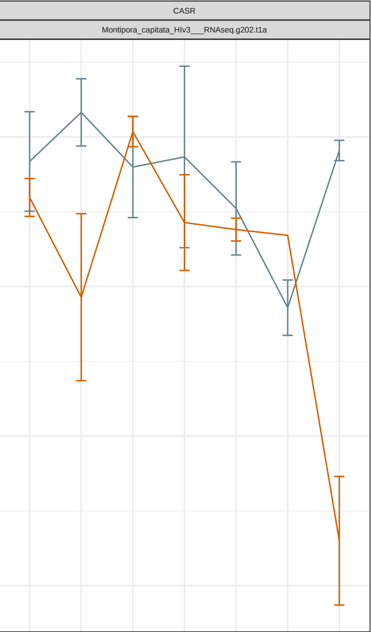
Cluster 2
