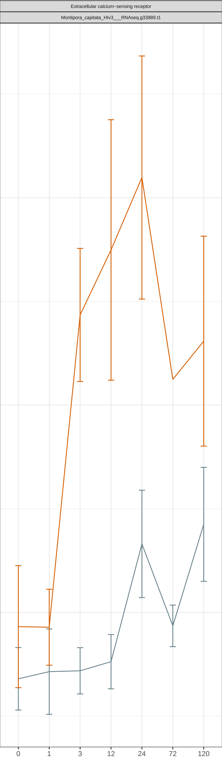
Cluster 4
