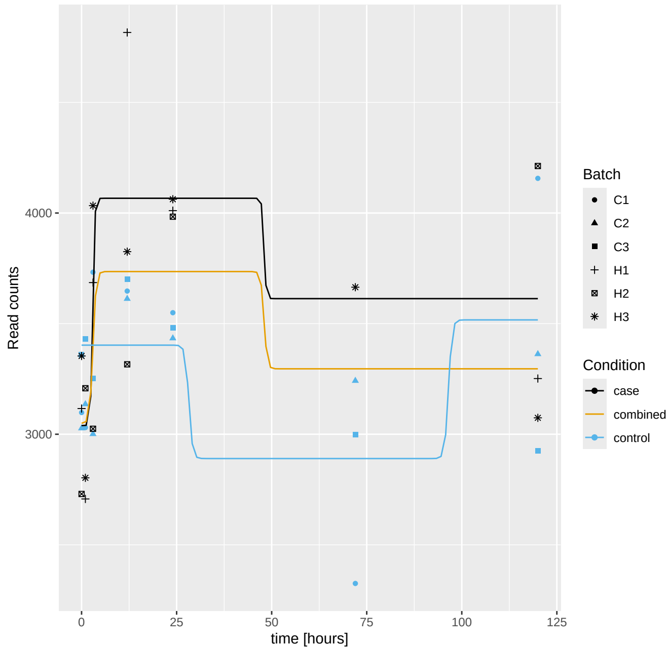
Montipora_capitata_Hlv3___RNAseq.g30015.t1b: log10 q = 0
