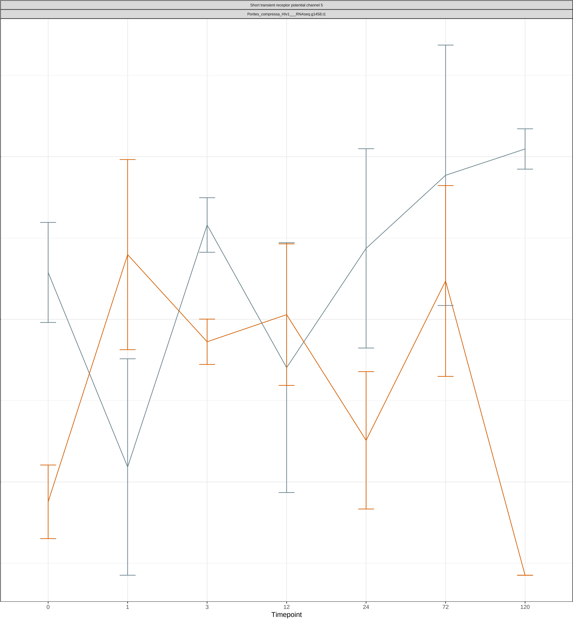
Cluster 4
