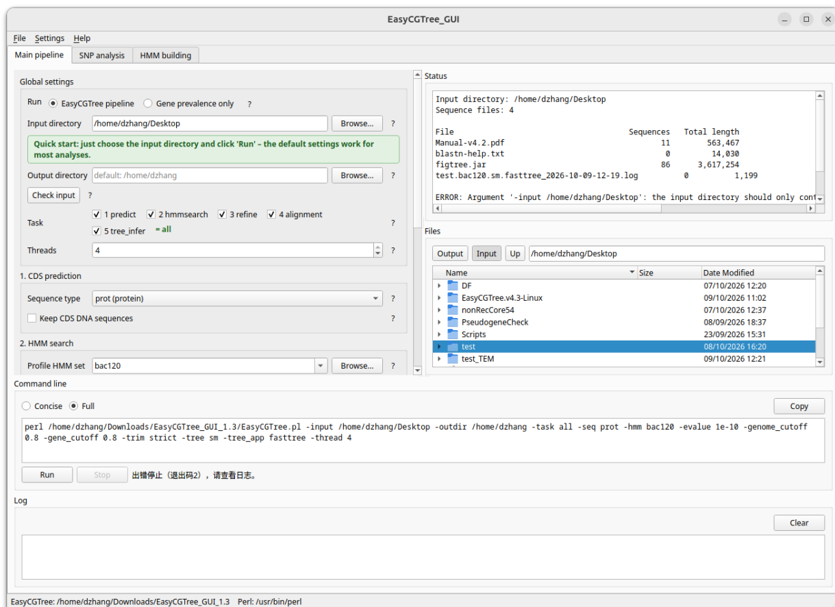
Fig. 1 The main window of EasyCGTree_GUI
