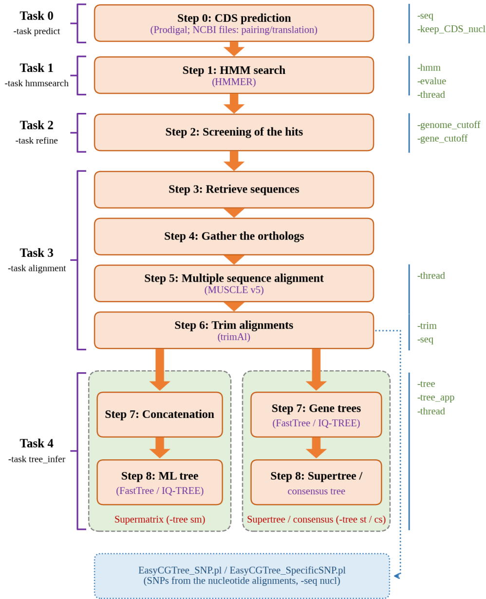
Fig. 2 Program flowchart of EasyCGTree for a complete run
