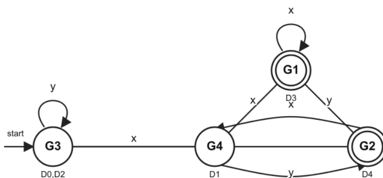
Minimal DFA: (x|y)^* x (x|y)
