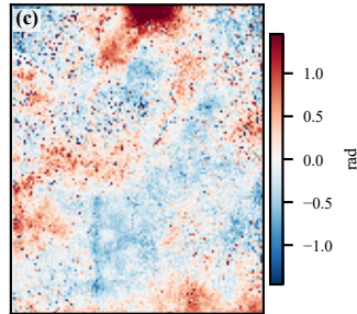
HOMA-DEM correction
