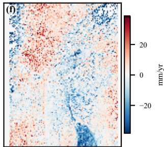
MintPy-corrected velocity
