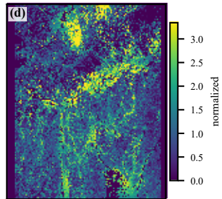
HOMA observability
