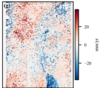
HOMA-corrected velocity
