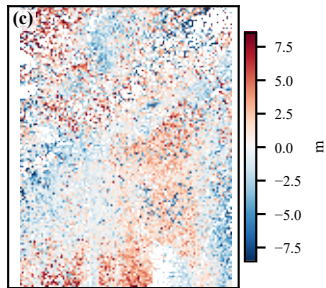
HOMA - MintPy (offset removed)
