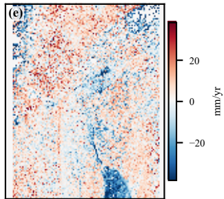
Velocity before DEM correction
