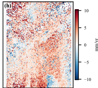
HOMA - MintPy velocity
