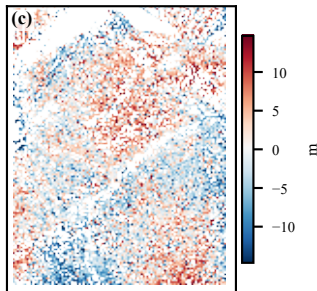
HOMA - MintPy (offset removed)
