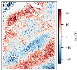
Velocity before DEM correction
