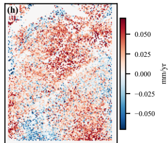
HOMA - MintPy velocity
