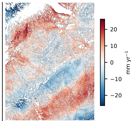
d MintPy velocity
