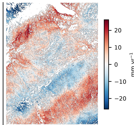
e Huber-corrected velocity
