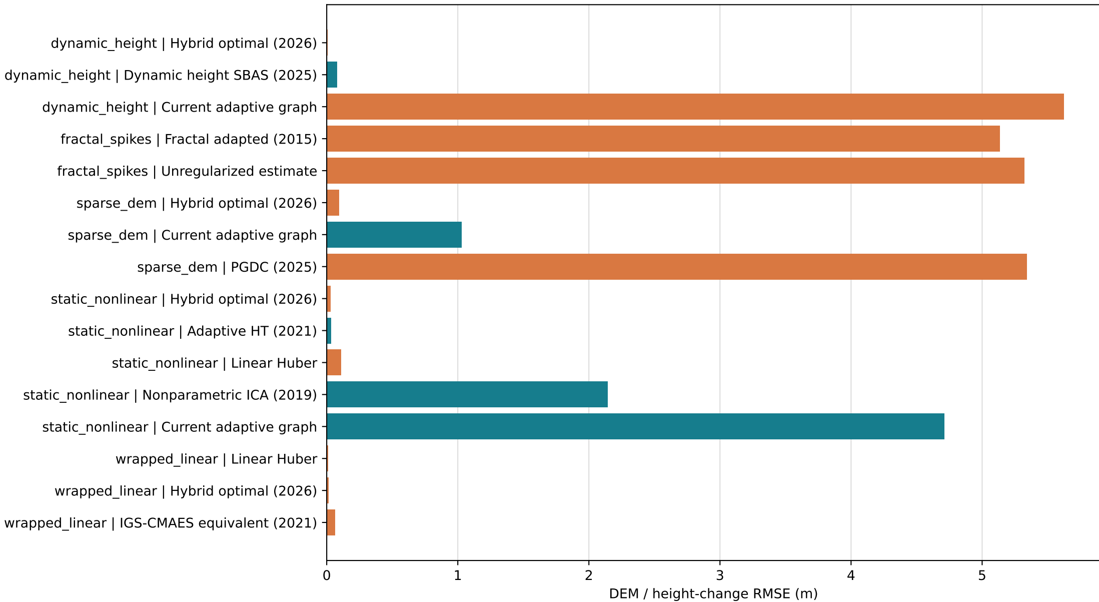
RMSE is comparable only within the same scenario
