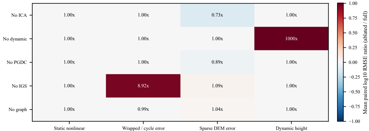
HOMA-DEM module ablation
