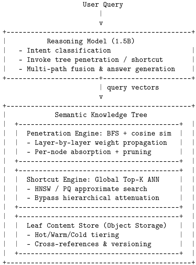
Figure 1: Tree-KB system architecture showing the separation of indexing (tree) and reasoning (small model).
