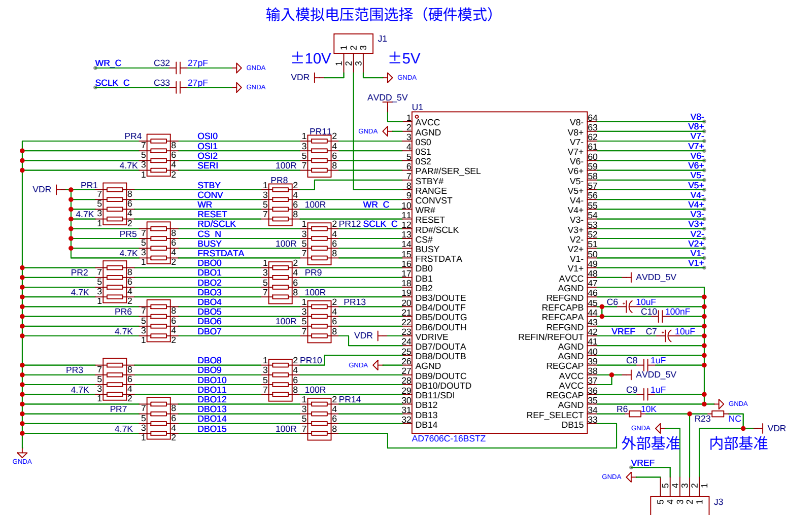
AD7606C
