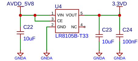
5.8V转3.3V
