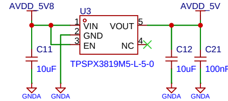
5.8V转5V
