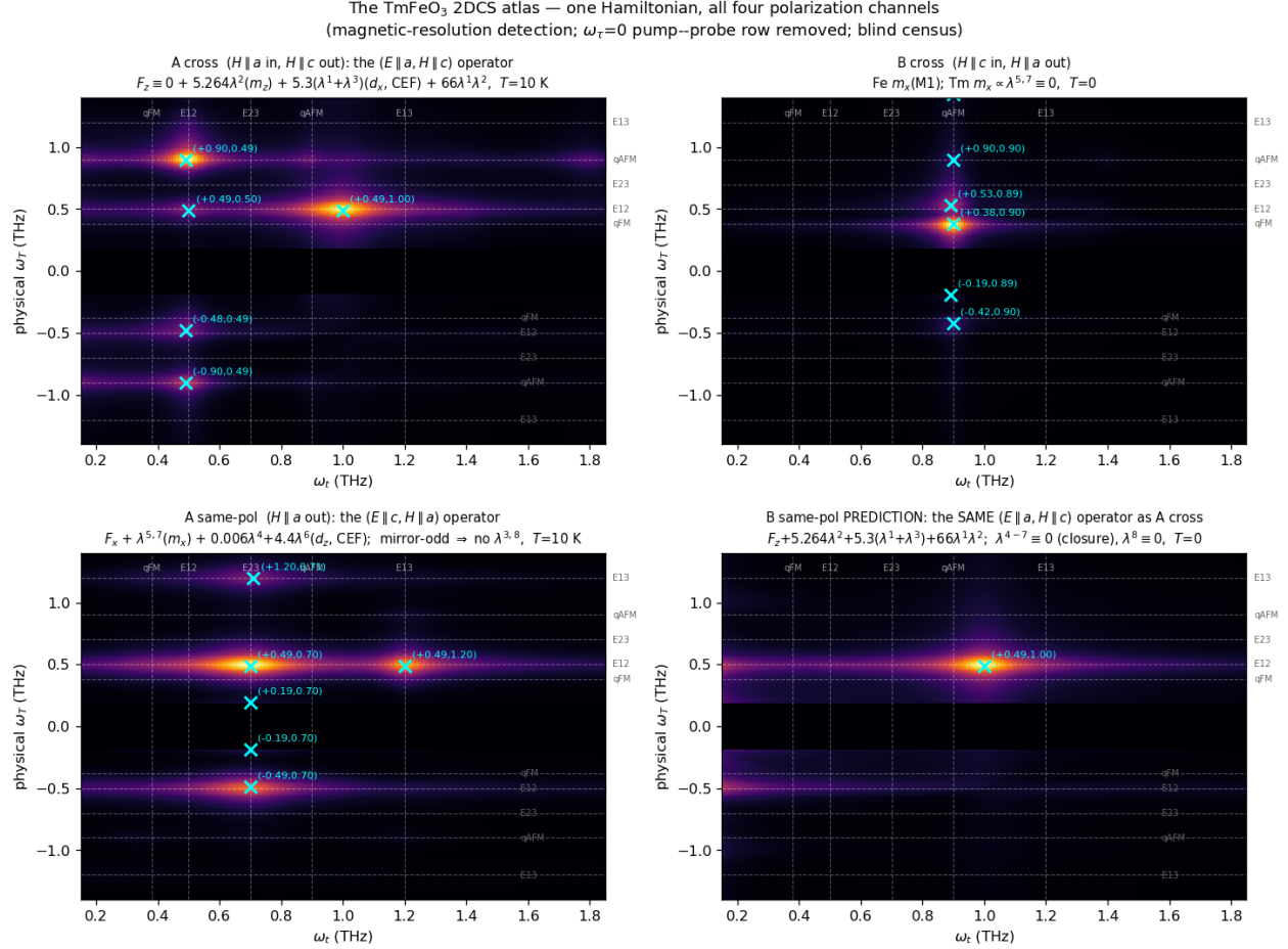
Figure S9: All four polarization channels from the single consolidated Hamiltonian, regenerated with the final methods. Only two detection operators appear, one per analyser polarization state, each containing both the magnetic and the electric dipole that radiate into it (section S11.1); the \tau -averaged signal is subtracted per detection time so the \omega_\tau = 0 pump–probe row is removed, with |\omega_T| < 0.18 \text{ THz} masked; blind census, crosses. Top left: geometry-A cross, the ( E \parallel a, H \parallel c ) operator F_z \equiv 0 + \mu\lambda^2 + w_{E1}(\lambda^1 + \lambda^3) + \beta\lambda^1\lambda^2 — the ( q_{\text{AFM}}, E_{12} ) peak of W_1^{yy} and the 2E_{12} harmonic. Top right: geometry-B cross, the ( E \parallel c, H \parallel a ) operator with its Tm part identically zero — ( q_{\text{FM}}, q_{\text{AFM}} ) and the \kappa^B -gated ( E_{12}, q_{\text{AFM}} ). Bottom left: geometry-A same-polarized, the same ( E \parallel c, H \parallel a ) operator, CEF composite at 10 K; both its constituents are mirror-odd, so it carries no population term. Bottom right: the geometry-B same-polarized prediction , analysed with the same operator as top left — led by the 2E_{12} harmonic, with the rectified \lambda^3 population pair at \omega_t \rightarrow 0 beneath it. Numerical censuses in data/census_atlas_final.json .
