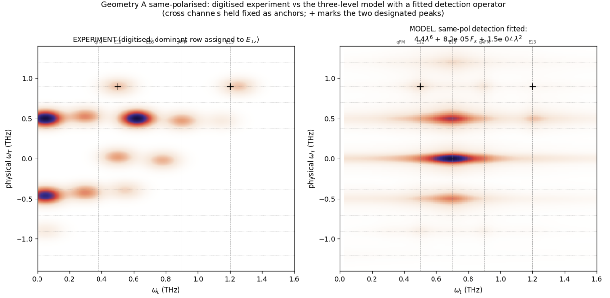
Figure 9: Digitised measurement (left) against the model with the three symmetry-required detection weights fitted (right), same axes and colour scale. Crosses mark the two designated peaks. Four of the six measured amplitudes are reproduced within 15% (section 19.5).
