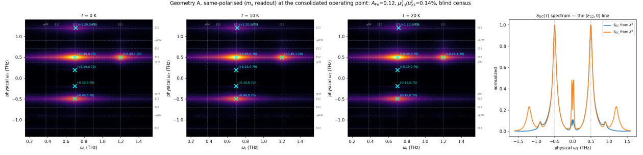
Figure 8: Geometry-A same-polarised channel at 0, 10 and 20 K, with the S_{DC}(\tau) panel in which the rectified (E_{12}, 0) line appears at +0.49 THz. The census is stable across this temperature range.
