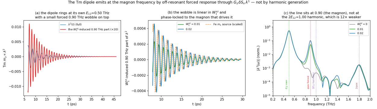
Figure 10: Why the Tm dipole emits at the magnon frequency: it is an off-resonant forced response through G_z \delta S_x \lambda^1 , not harmonic generation. (a) the dipole rings at its own E_{12}=0.50 THz with a small forced 0.90 THz wobble on top; (b) that wobble grows linearly with W_1^{xz} and is phase-locked to the magnon that drives it; (c) the line sits at 0.90 (the magnon), not at the 2E_{12}=1.00 harmonic, which is 12× weaker.
