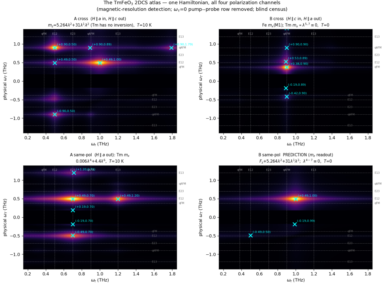
Figure 7: The atlas: all four polarisation channels from one Hamiltonian at one operating point. Detection is resolved by the emitted magnetic polarisation, so each panel reads one Cartesian moment component (section 19.2). Dashed guides mark the five mode energies; cyan crosses are blind-census maxima; the \omega_r = 0 pump-probe row is removed.
