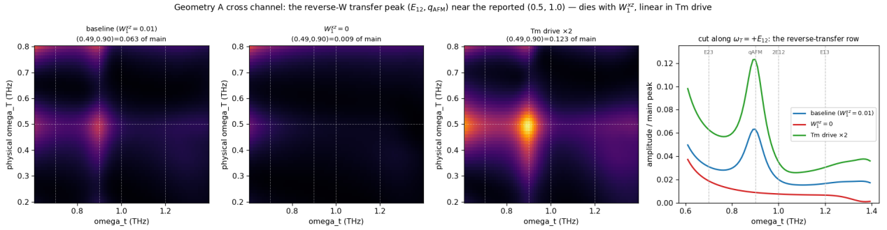
Figure S3: The reverse- W transfer peak in the geometry-A cross channel ( \lambda^2 ), zoomed on the region of the reported (0.5, 1.0) feature; all amplitudes normalized to the main ( q_{\text{AFM}}, E_{12} ) peak. Left to right: baseline (genuine local maximum at (+0.49, 0.90) = 0.063 ), W_1^{xz} = 0 (collapsed to 0.009), Tm drive \times 2 (doubled to 0.123). Rightmost: the \omega_T = +E_{12} row cut—the peak sits at the q_{\text{AFM}} emission frequency with the 2E_{12} = 1.00 THz harmonic as a shoulder.
