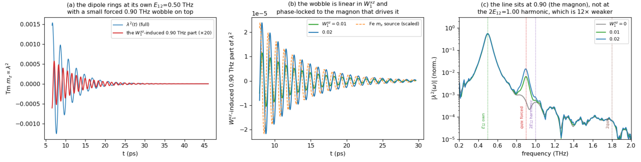
Figure S4: Time evolution of the Tm m_z dipole. (a) It rings at its own E_{12} = 0.50 THz, with a small forced 0.90 THz wobble on top (the W_1^{yz} -induced part, \times 20 ). (b) Isolating that part by differencing runs at W_1^{yz} = 0, 0.01, 0.02 : it grows linearly with the coupling and is phase-locked to the Fe m_x magnon that drives it. (c) Spectrum: the line sits at the magnon frequency 0.90 THz, not at the 2E_{12} = 1.00 THz harmonic, which is present but 12\times weaker; the 2q_{\text{AFM}} = 1.80 THz line from the quadratic W_1^{yy} vertex is weaker still.
