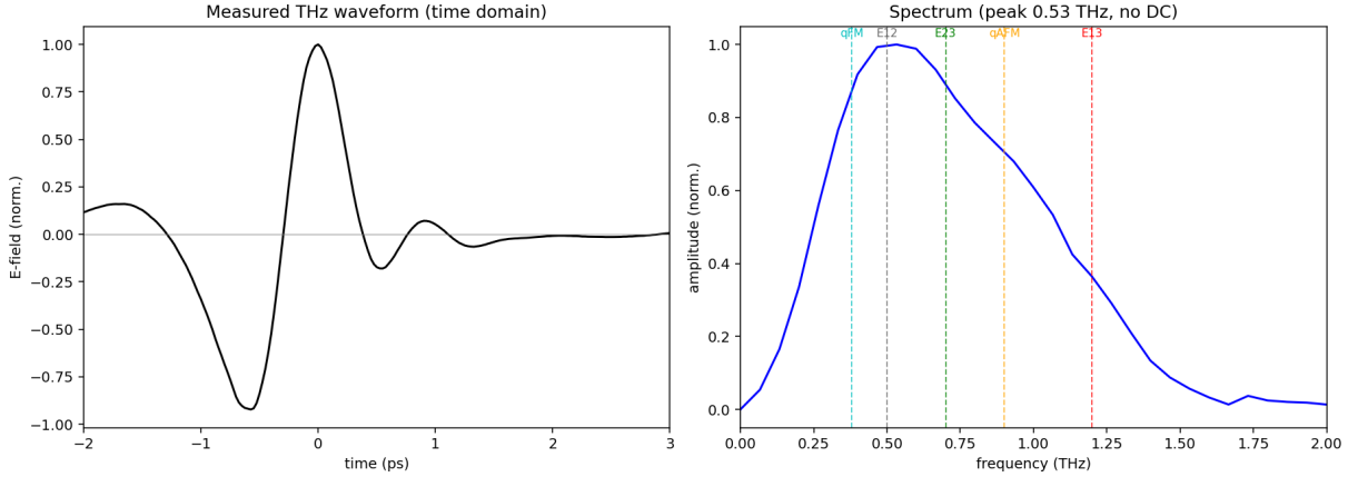
Figure S1: The measured THz pump. Left: single bipolar cycle ( \sim 1.2 \text{ ps} , no DC). Right: amplitude spectrum peaked at 0.53 \text{ THz} \approx E_{12} , covering all five modes. The absence of DC content removes the quasistatic-tilt legs that a Gaussian stand-in pulse would add; the measured waveform is the cleanest configuration.
