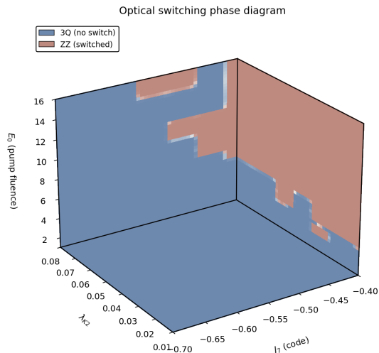
FIG. 1. Clean driven phase diagram at the tuned-Kruger point. The clean system is the control problem: it has a comparatively sharp threshold between a stable 3Q response and a zigzag-like written state. This cube fixes the microscopic switching physics that the large-cell disorder calculations broaden.
