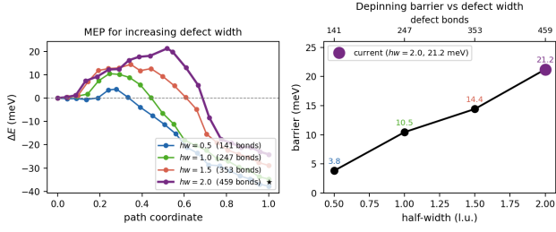
FIG. 3. Kinetic barrier of the hard-fault defect as a function of band width. (Left) Climbing-image geodesic MEP curves for four defect half-widths ( hw = 0.5, 1.0, 1.5, 2.0 ; 141, 247, 353, 459 defect bonds) at fixed \delta K = -0.5|K| . The path runs from the pinned zigzag strip to relaxed 3Q with the defect present; energies are shifted so the zigzag endpoint lies at zero. (Right) Converged barrier height versus half-width. The barrier grows monotonically from 3.8 meV at hw = 0.5 to 21.2 meV at the operating point hw = 2 (star), which is safely above the 18.96 meV lifetime target. The relaxed 3Q endpoint sits 24.15 meV below the pinned strip at the operating point, confirming metastability.
