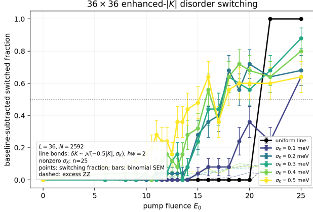
FIG. 4. Large-cell switching-fraction check on a 36 \times 36 honeycomb lattice ( N = 2592 spins). The calculation uses the same enhanced- |K| line as the lifetime MEP: selected bonds in a hw = 2 vertical band have the fixed offset \delta K_{\text{line}} = -0.5|K| , while all nearest-neighbor bonds also receive zero-mean background disorder \delta K_{\text{bg}} \sim \mathcal{N}(0, \sigma_K) . All geometry, reference states, disorder files, driven MD runs, and quenches are regenerated on the 36 \times 36 solver lattice. The displayed pump range covers the broadened onset of the fixed-line/global-disorder protocol. Nonzero-disorder curves use twenty-five seeds; error bars in Fig. 2(c) denote the binomial standard error of the switching fraction.
