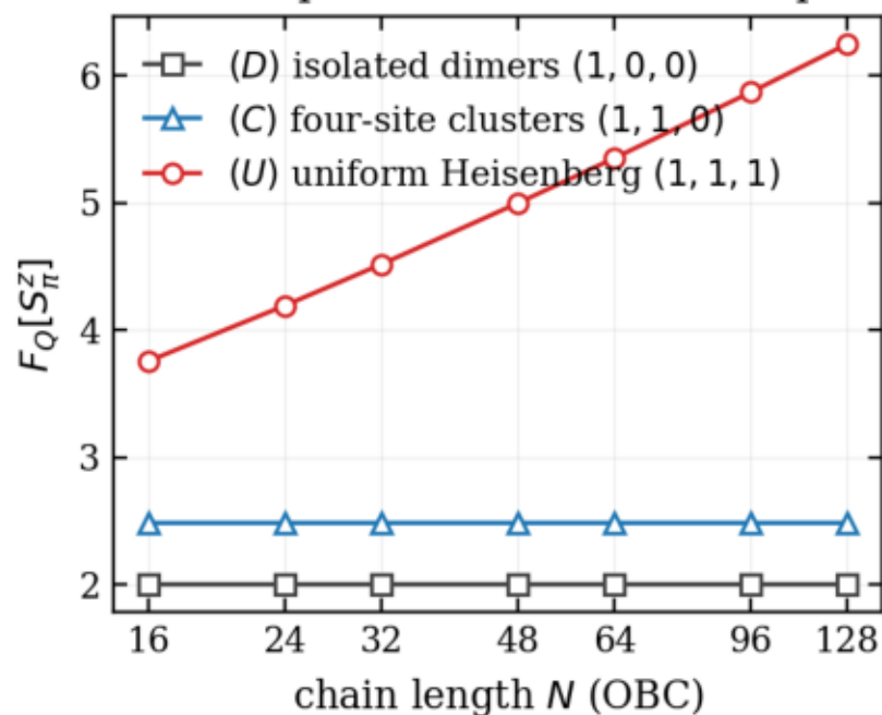
Corrected period-4 chain: anchor points
