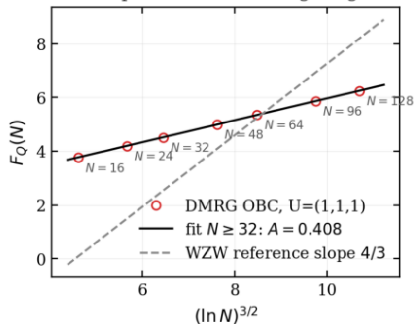
Uniform point: WZW scaling diagnostic
