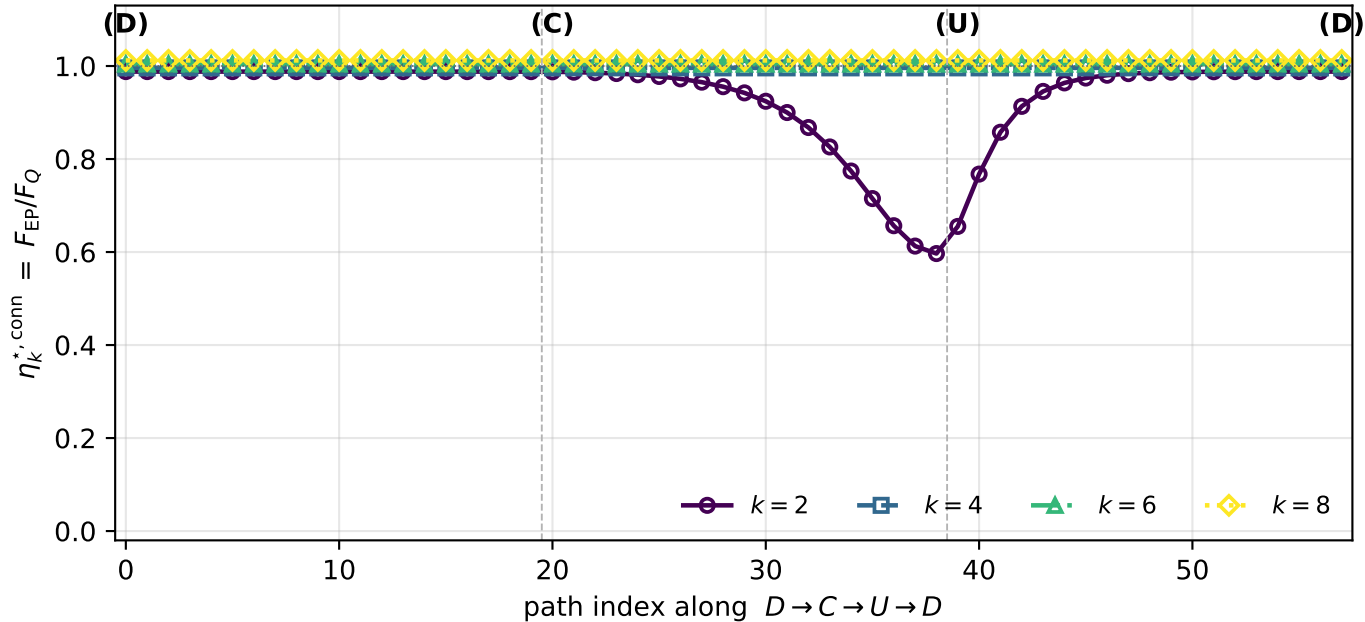
Connected-subspace matched-filter saturation, J_1 - J_2 - J_3 chain ( N = 8 )
