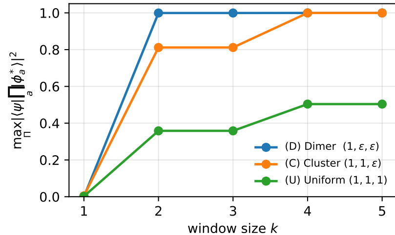
(c) Best k -producible product fidelity
