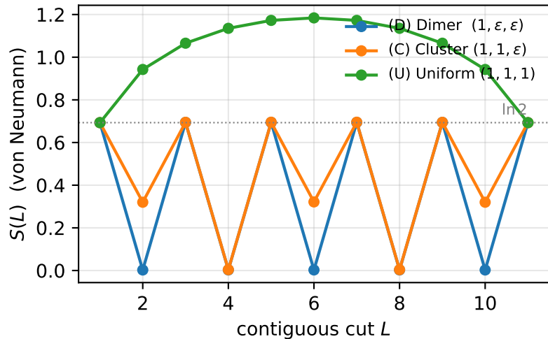
(a) Bipartite entropy, N = 12
