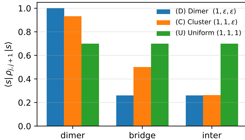
(b) Singlet fidelity by bond class
