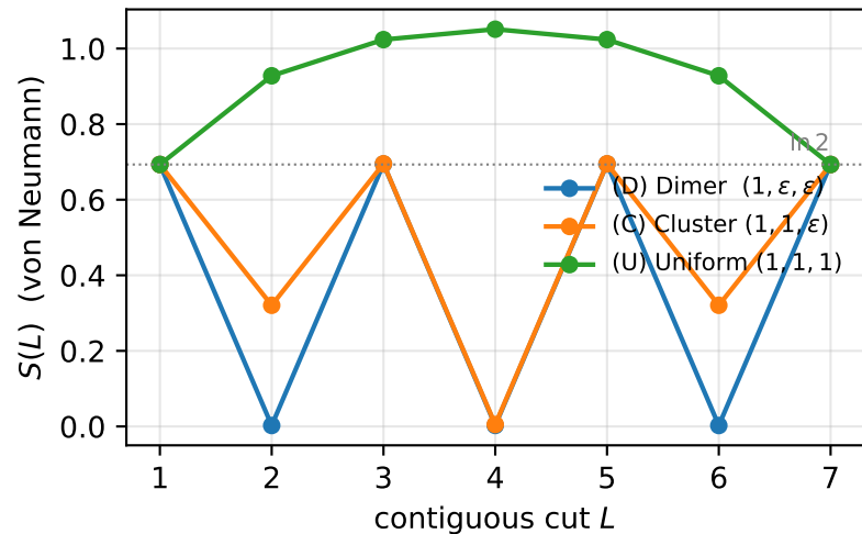
(a) Bipartite entropy, N = 8
