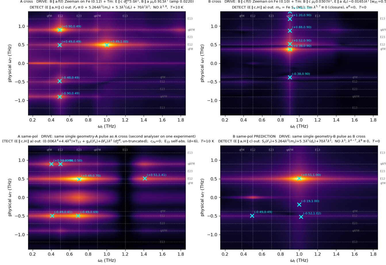
FIG. 1. The atlas: four polarisation channels from one Hamiltonian at one operating point. Dashed guides mark the five mode energies; crosses are blind-census maxima; the \omega_T = 0 row is removed.
