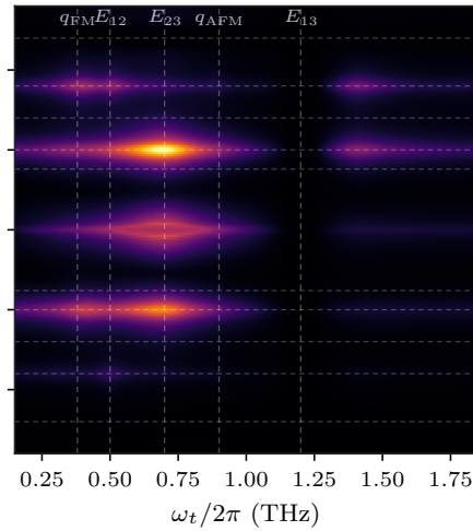
T=10 K
