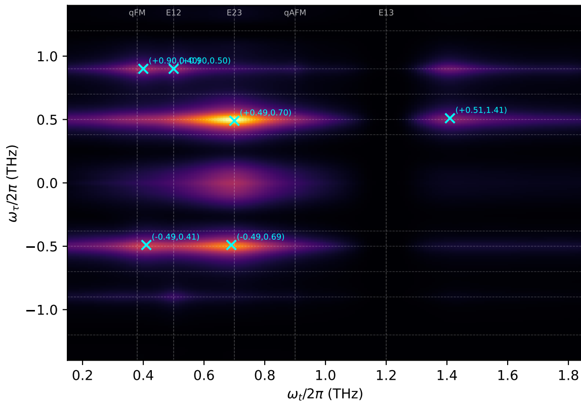
(c) A same-pol O_1 \rightarrow O_1
