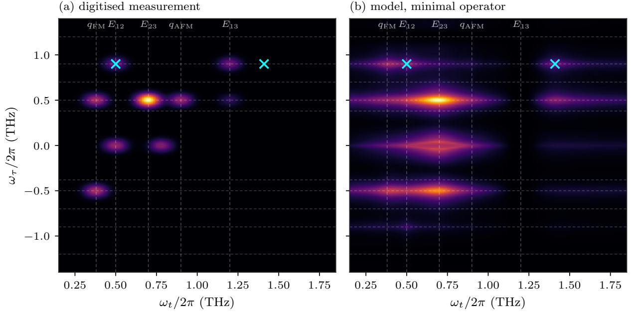
Figure 9: Digitised measurement (a) against the model with the minimal operator (b), same axes and colour scale. Crosses mark the two designated (“+”) q_{AFM} -row peaks; the model places the high tone at q_{AFM}+E_{12} = 1.41 THz (the digitisation, at \pm 0.05 THz, had anchored it to the nearby E_{13} guide). Six of nine amplitudes agree within 15% (section 19.5).
