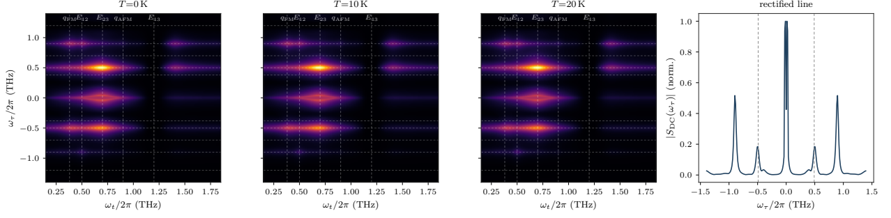
Figure 8: Geometry-A same-polarised channel at 0, 10 and 20 K, with the S_{DC}(\tau) panel in which the rectified ( E_{12}, 0 ) line appears at +0.49 THz. The census is stable across this temperature range.
