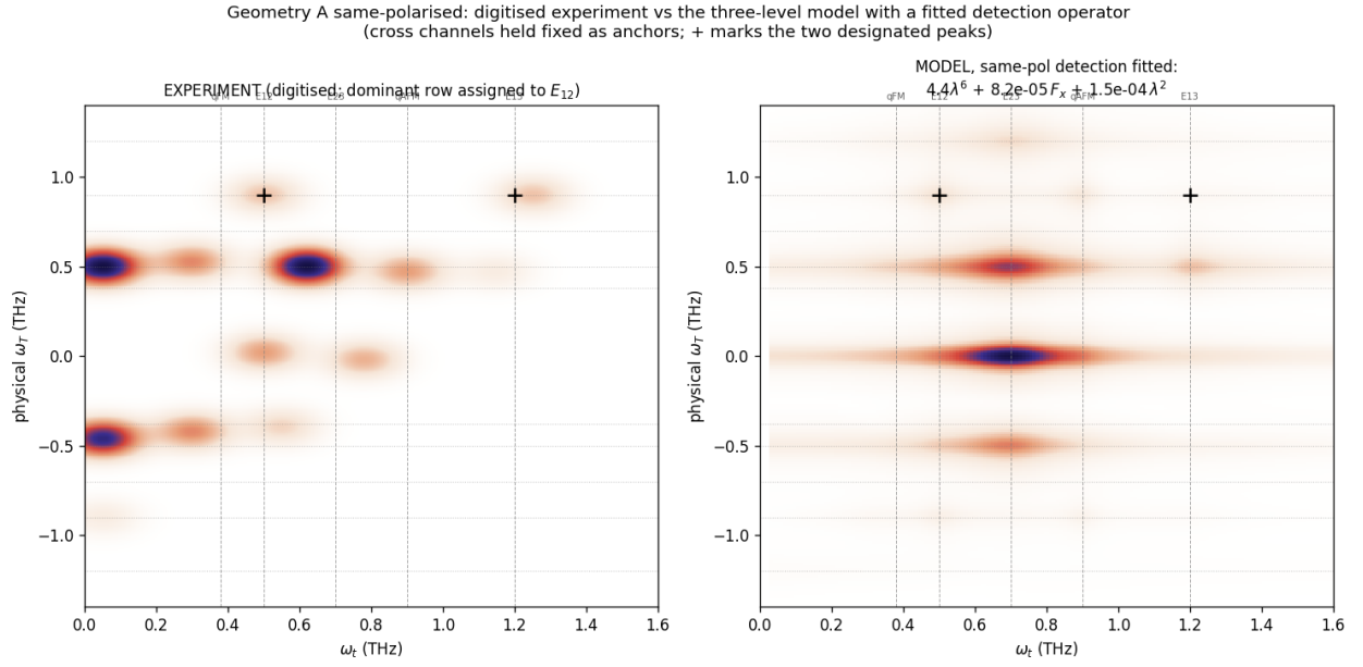
Figure 9: Digitised measurement (left) against the model (right), same axes and colour scale: two symmetry-required detection weights fitted, the Fe weight bounded by the absent magnon diagonal. Crosses mark the two designated peaks. Four of the six measured amplitudes are reproduced within 15% (section 19.5).
