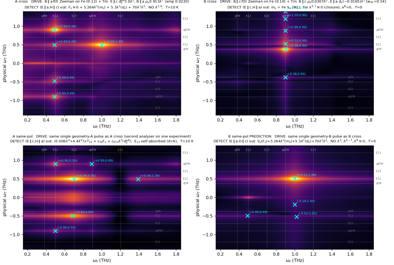
FIG. 1. The atlas: four polarisation channels from one Hamiltonian at one operating point. Dashed guides mark the five mode energies; crosses are blind-census maxima; the \omega_\tau = 0 row is removed.
