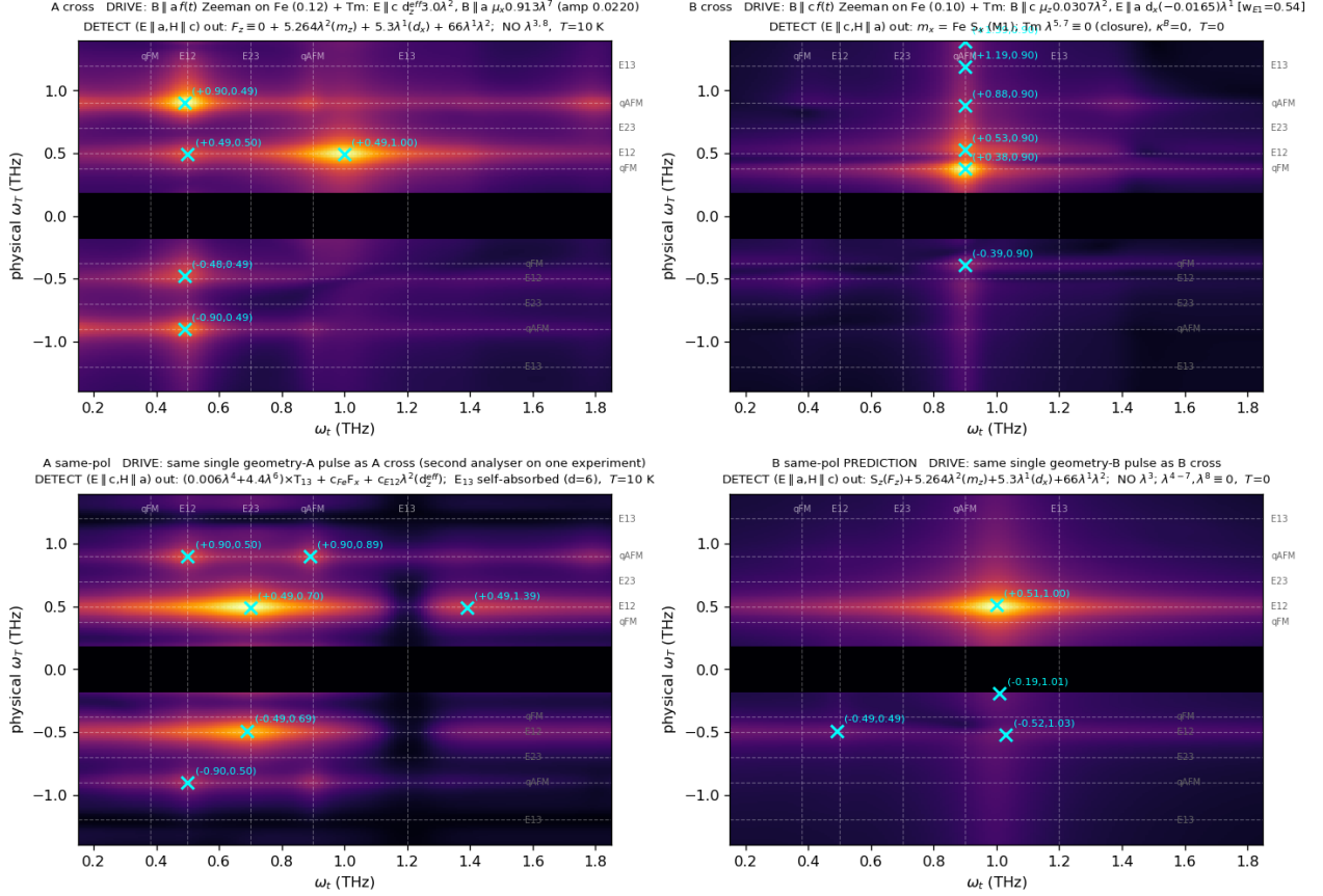
The \text{TmFeO}_3 2DCS atlas — \kappa^B -FREE scenario: one Hamiltonian (all-static Fe-Tm vertices), one physical pulse per geometry (geometry-B coherence written electrically via d_x , converted by master W_1^z ; \omega_\tau=0 row removed; blind census; amplitude 0.45 colour scale)
