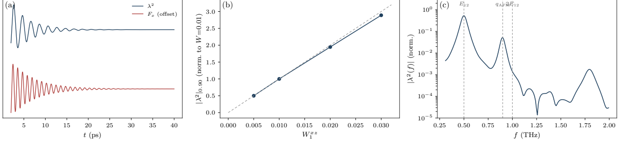
Figure 10: Why the Tm dipole emits at the magnon frequency: an off-resonant forced response through the static family, not harmonic generation. (a) Pump-only trajectories of \lambda^2 and F_x (offset): the dipole rings at its own E_{12} with a small 0.90 THz component on top. (b) The 0.90 THz content of \lambda^2 grows linearly with W_1^{xz} through the origin (dashed: exact linearity). (c) The \lambda^2 spectrum: the sideband sits at the magnon frequency, distinct from the 2E_{12} = 1.00 harmonic; the weak feature near 1.8 THz is the predicted 2q_{\text{AFM}} line.
