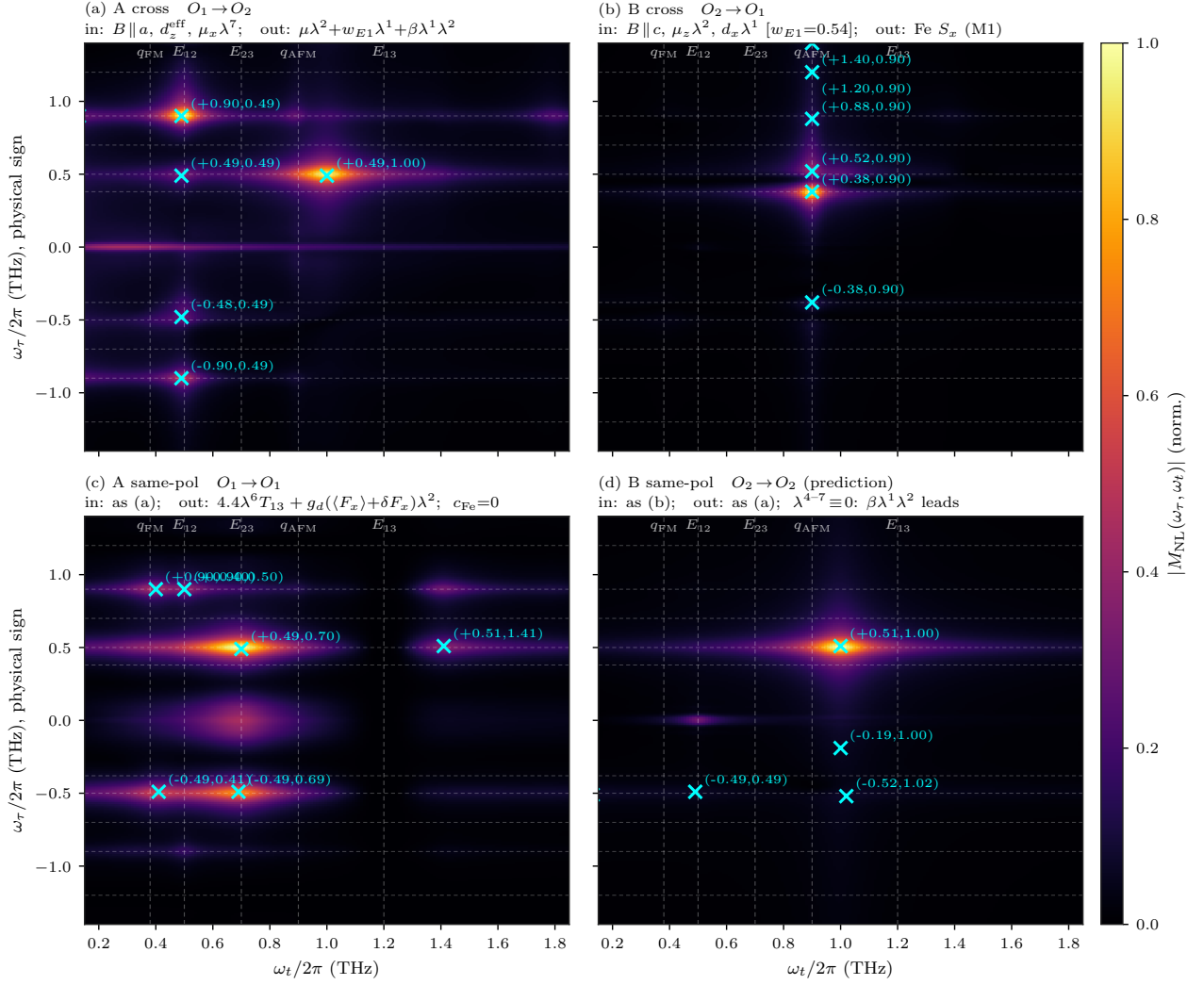
Figure 7: The atlas: all four polarisation channels from one Hamiltonian at one operating point. Detection is resolved by the emitted magnetic polarisation, so each panel reads one Cartesian moment component (section 19.2). Dashed guides mark the five mode energies; cyan crosses are blind-census maxima; linear amplitude colour scale; the \omega_\tau = 0 pump-probe row is retained in the geometry-A panels (auto-scaled to the measured relative amplitude) and excluded from the census.
