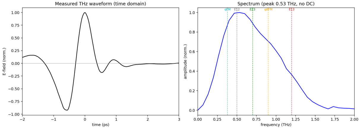
Figure S1: The measured THz pump. Left: single bipolar cycle ( \sim 1.2 ps, no DC). Right: amplitude spectrum peaked at 0.53 THz \approx E_{12} , covering all five modes. The absence of DC content removes the quasistatic-tilt legs that a Gaussian stand-in pulse would add; the measured waveform is the cleanest configuration.
