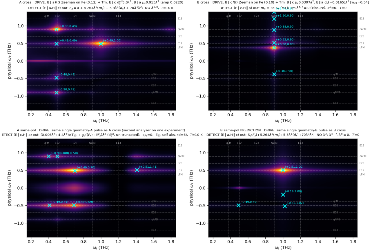
Figure S3: All four polarisation channels from the single consolidated Hamiltonian at one operating point (linear amplitude colour scale; blind-census crosses; the \omega_\tau = 0 pump–probe row retained in the geometry-A panels, auto-scaled, and excluded from the census). Each panel states its exact drive and detection. Numerical censuses in data/census_atlas_kBfree.json .
