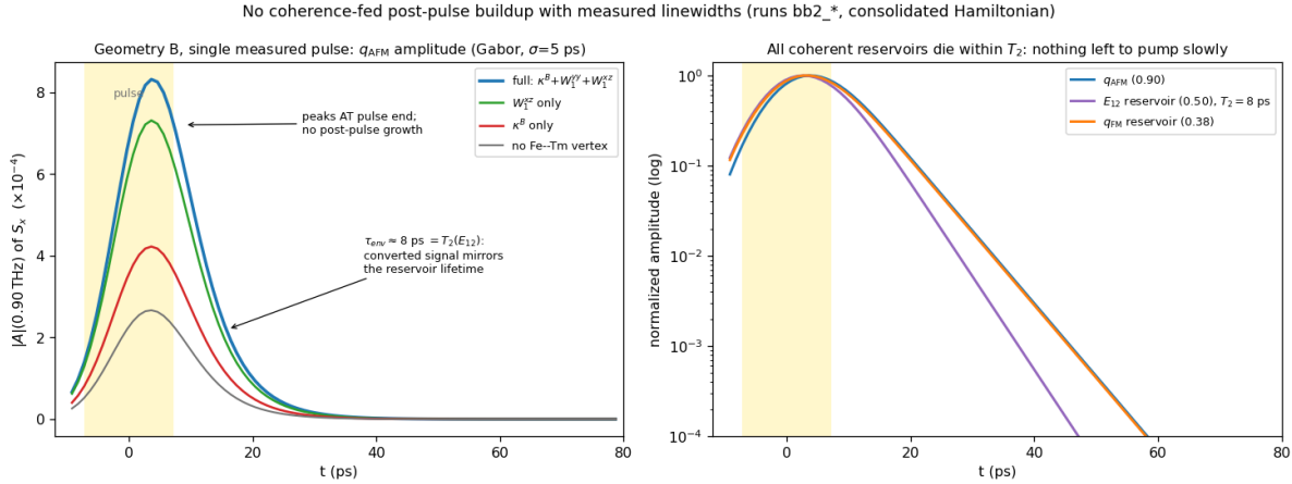
Figure S2: No coherence-fed post-pulse buildup once the measured linewidths are enforced (single measured pulse, geometry B; Gabor amplitude, \sigma = 5 ps). Left: the q_{\text{AFM}} amplitude peaks at pulse end and decays with \tau_{\text{env}} \approx 8 ps = T_2(E_{12}) ; the vertices set the absolute scale but none produces post-pulse growth. Right: all coherent reservoirs die within their measured T_2 (log scale)—there is nothing left to pump the magnon slowly.
