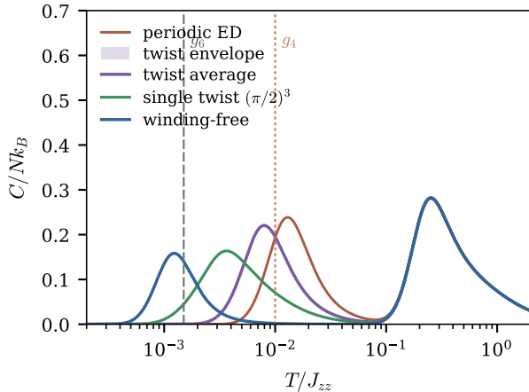
(b) C(T) at J_{\pm}/J_{zz} = -0.05
