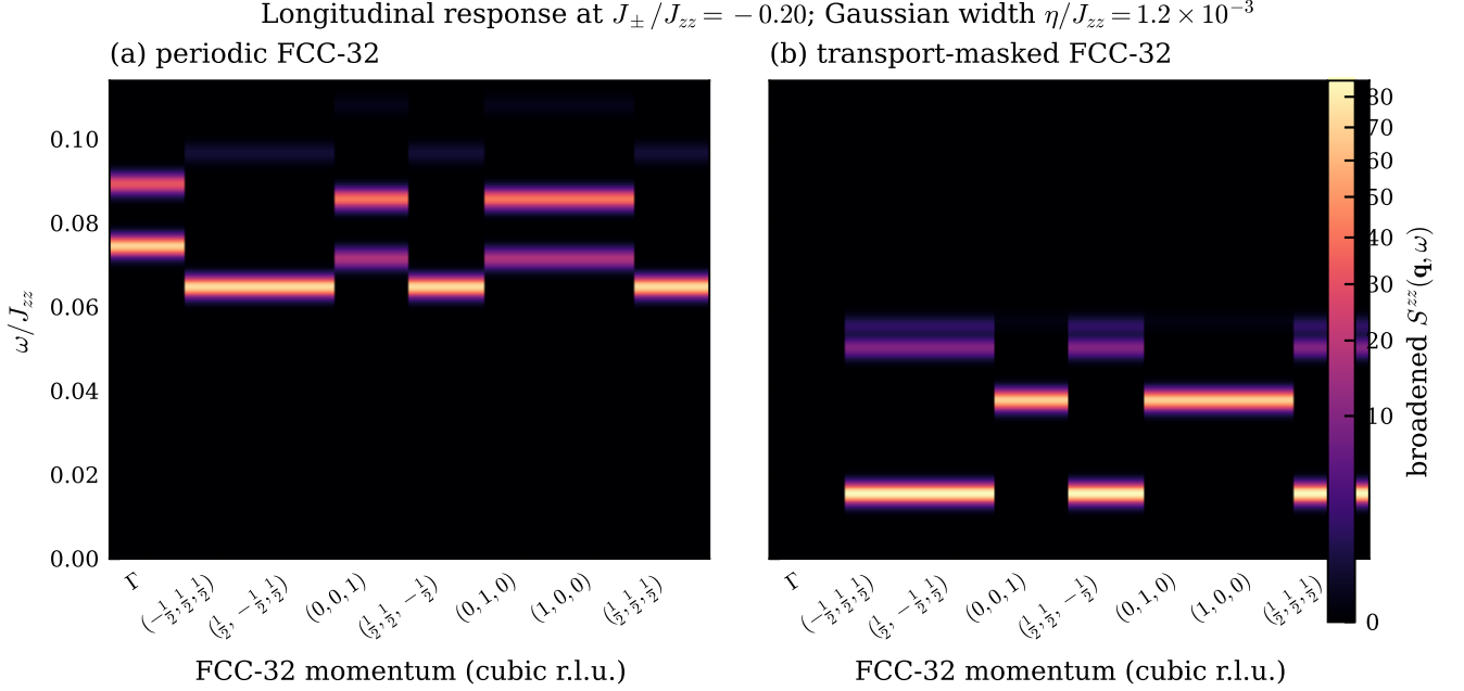
FIG. 2. Longitudinal dynamical structure factor at all eight FCC-32 momenta for J_{\pm}/J_{zz} = -0.20 . (a) Naive periodic dynamics and (b) the transport-masked theory use the same depth- d = 1 space, 120 final states, four sublattice probes, Gaussian width \eta/J_{zz} = 1.2 \times 10^{-3} , and common color scale. Periodic dynamics produces strong inelastic response at \Gamma and a higher apparent excitation scale. The mask removes the \Gamma response while retaining finite weight at every nonzero momentum.
