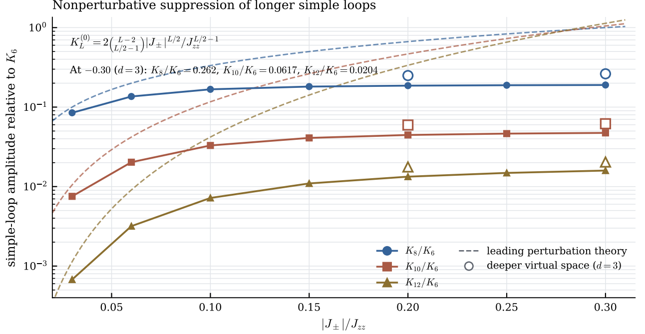
FIG. 3. FCC-32 simple-loop hierarchy. Solid symbols are the complete virtual-depth- d=2 results; open symbols are matched virtual-depth- d=3 checks. Dashed curves are the leading ratios in Eq. (13). Bare perturbation theory predicts that the longer loops approach or exceed the hexagon near |J_{\pm}|/J_{zz} = 0.30 ; the nonperturbative Feshbach amplitudes flatten far below it.
