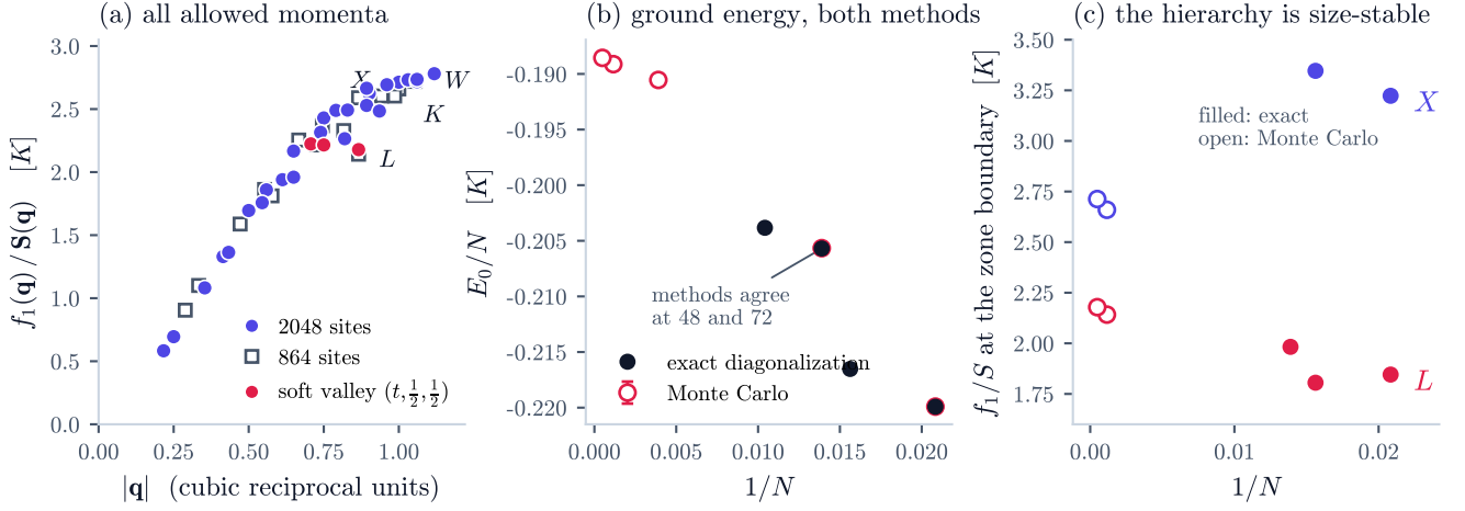
FIG. 6. Thermodynamic evidence, with the numerical checks displayed rather than asserted. (a) The Feynman ratio f_1/S at every allowed momentum star of the 2048-site supercell (filled circles, with statistical error bars from binned Monte Carlo averages; symmetry copies of each star agree to better than 0.04 and are merged), overlaid with the 864-site values (open squares). No path or interpolation is involved: each point is a true eigenmode weight. The zone-boundary minimum is at L ; red marks the shallow soft valley along (t, \frac{1}{2}, \frac{1}{2}) (Sec. XII A). (b) Ground-state energy per site against 1/N : exact diagonalization (filled) and Green's-function Monte Carlo (open, with error bars) on one axis. At the two sizes where both methods exist, 48 and 72 sites, they agree within statistical errors — the method gate, shown explicitly. (c) The ratio at L and X across both methods and all sizes: the zone-boundary hierarchy, L softest, holds at every size, while the interior of the zone (not shown) drifts strongly — the reason large systems were required.
