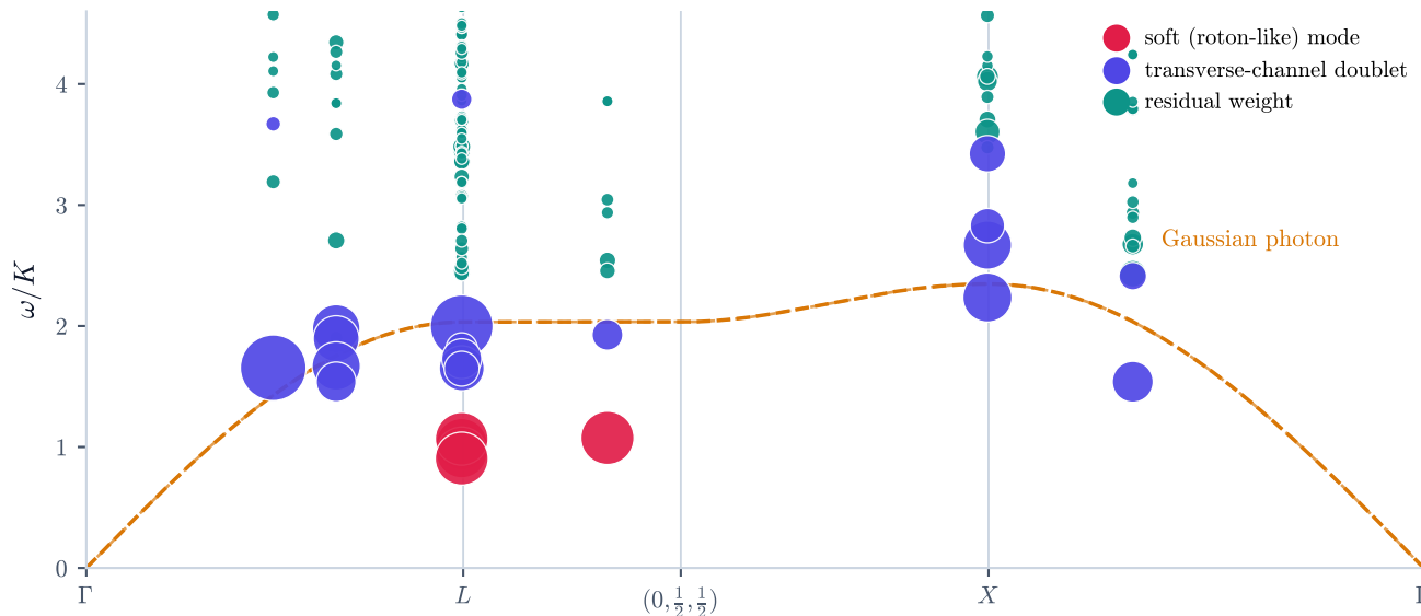
FIG. 2. The S^z spectrum as a dispersion relation. Every resolved pole of the diagonalized clusters (complete diagonalization at 48 sites, Lanczos-converged at 64, 72 and 96, overlaid) whose momentum lies on the path \Gamma \rightarrow L \rightarrow (0, \frac{1}{2}, \frac{1}{2}) \rightarrow X \rightarrow \Gamma , placed at its true position; marker area is the level's share of S(\mathbf{q}) at its momentum. Red: the soft roton-like level; indigo: the two dominant transverse-channel levels; teal: residual weight beyond the two dominant levels (its multiparticle versus magnetic character is discussed in the text). The dashed curve is the Gaussian photon, evaluated analytically on the infinite lattice along the same path with its single fitted scale; the analytic curl reproduces the cluster singular value at L to machine precision. The spectrum tracks the free theory at long wavelength, and at L — and again at the soft-valley momentum (\frac{1}{6}, \frac{1}{2}, \frac{1}{2}) — reconstructs around a pole at roughly half the free-theory energy. The leg (0, \frac{1}{2}, \frac{1}{2}) \rightarrow X contains no cluster momentum and is shown for the free theory only.
