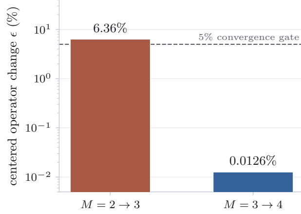
FIG. 1. Successive character-grid convergence of the exact cubic-16 band operator at (J_{\pm}, J_{\pm\pm})/J_{zz} = (0.046, 0) . Bars show the centered relative Frobenius change in Eq. (30) on a logarithmic axis, the two differing by nearly three decades; the dashed line is the preassigned 5% gate.
