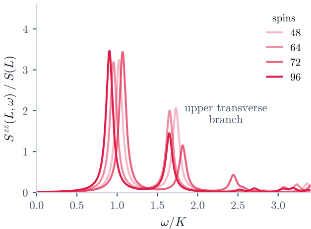
(b) the L spectrum at 48, 64, 72, 96 spins
