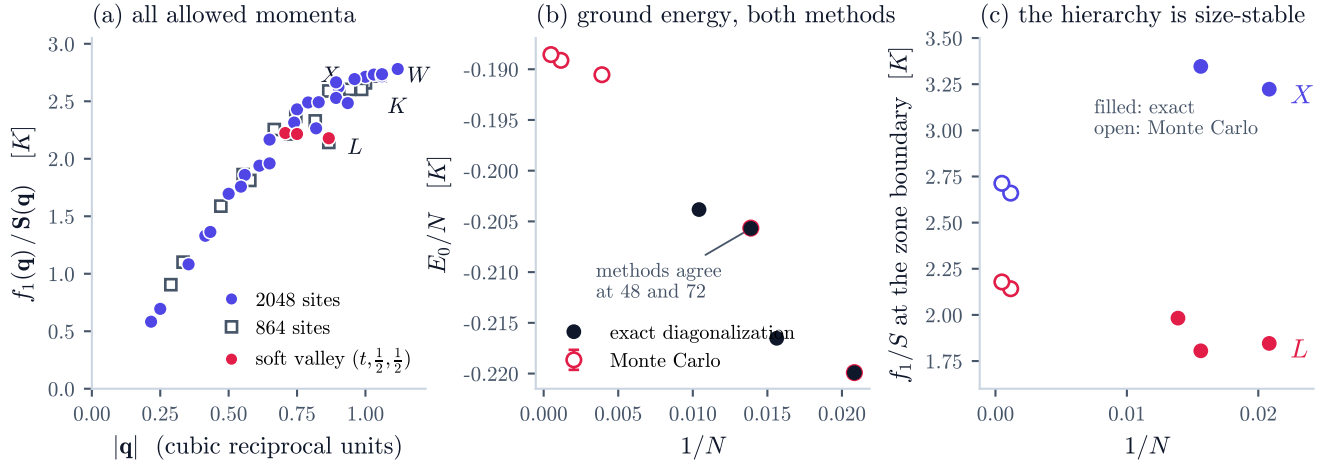
FIG. 5. Thermodynamic evidence, with the numerical checks displayed rather than asserted. (a) The Feynman ratio f_1/S at every allowed momentum star of the 2048-site supercell (filled circles, with statistical error bars from binned Monte Carlo averages; symmetry copies of each star agree to better than 0.04 and are merged), overlaid with the 864-site values (open squares). No path or interpolation is involved: each point is a true eigenmode weight. The zone-boundary minimum is at L ; red marks the shallow soft valley along (t, \frac{1}{2}, \frac{1}{2}) (Sec. XII A). (b) Ground-state energy per site against 1/N : exact diagonalization (filled) and Green's-function Monte Carlo (open, with error bars) on one axis. At the two sizes where both methods exist, 48 and 72 sites, they agree within statistical errors — the method gate, shown explicitly. (c) The ratio at L and X across both methods and all sizes: the zone-boundary hierarchy, L softest, holds at every size, while the interior of the zone (not shown) drifts strongly — the reason large systems were required.
