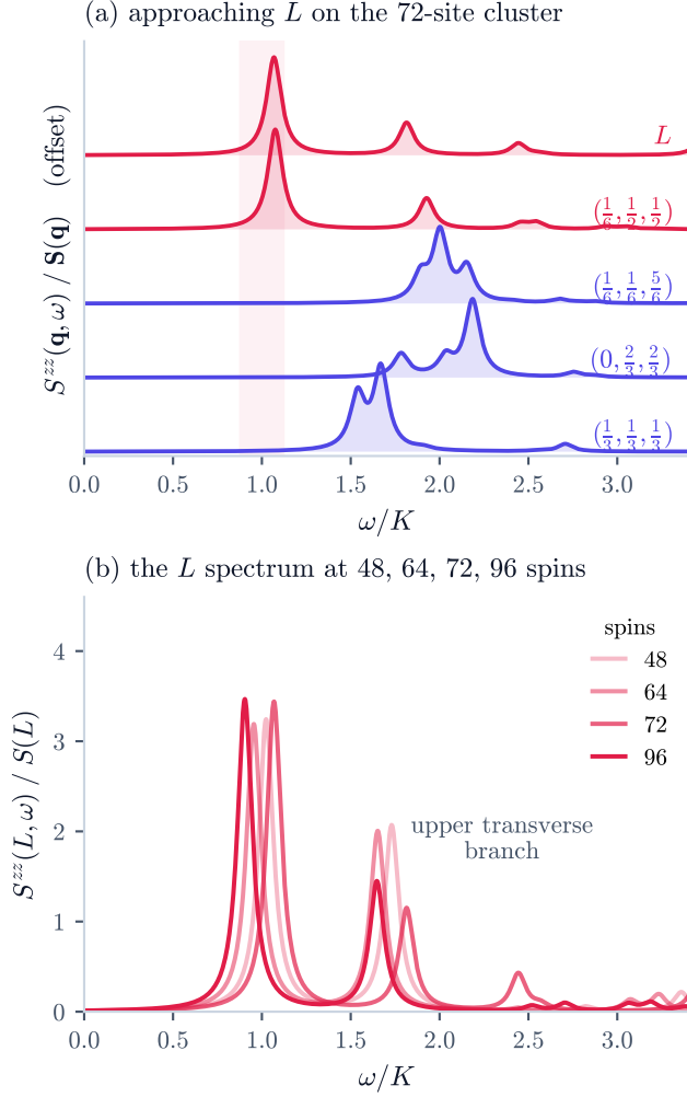
FIG. 2. The mode itself: exact S^{zz}(\mathbf{q}, \omega) near L . (a) The 72-site spectrum at five momenta, each normalized by its own S(\mathbf{q}) ; every pole is exact (Lanczos continued fraction with the sum-rule gate at 1.0000), broadened by a display-only \eta = 0.05K . At the three photon-like momenta the response peaks at 1.5–2.2K; at L and at the soft-valley momentum (\frac{1}{6}, \frac{1}{2}, \frac{1}{2}) (Sec. XII A) it collapses onto a single dominant pole near 1K carrying over half the weight (shaded band). (b) The L -point spectrum at all four diagonalized sizes, overlaid: the soft pole sits at 0.90–1.07K with about half the weight at every size, the upper transverse branch at 1.65–1.81K. Nothing here is fitted or extrapolated; the figure is the spectrum.
