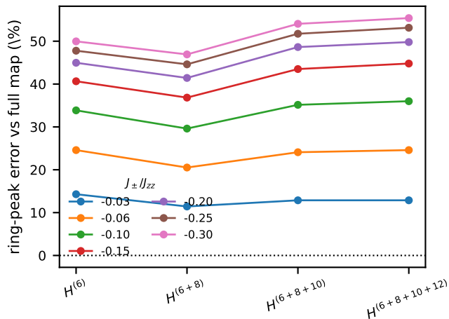
(b) the ladder does not converge
