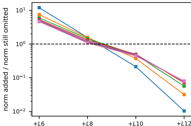
(c) past L = 8 the ladder adds less than it omits
