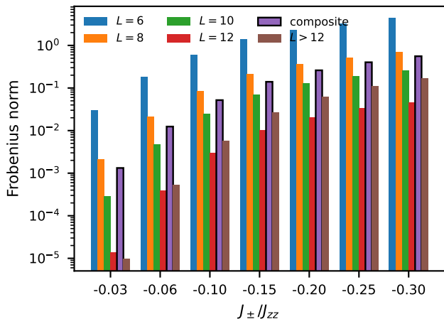
(a) norm budget: composite exceeds L = 10, 12
