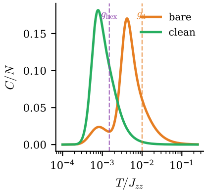
(a) 32 sites, J_{\pm} = -0.05
