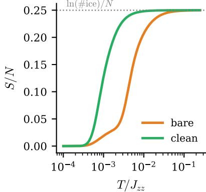
(c) photon entropy
