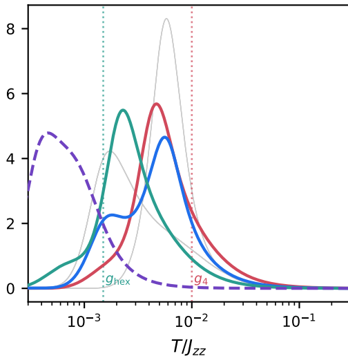
(b) 32-site FCC (PT), J_{\pm} = -0.05
