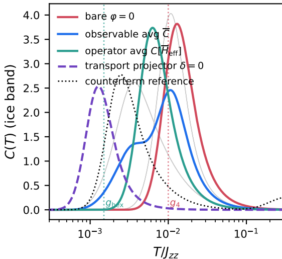
(a) 16-site cubic (exact), J_{\pm} = -0.05
