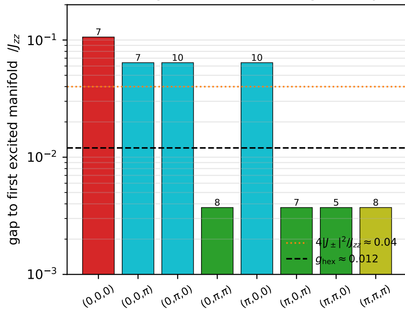
(b) gap above the quasi-degenerate ground manifold (label = ground-manifold degeneracy)
