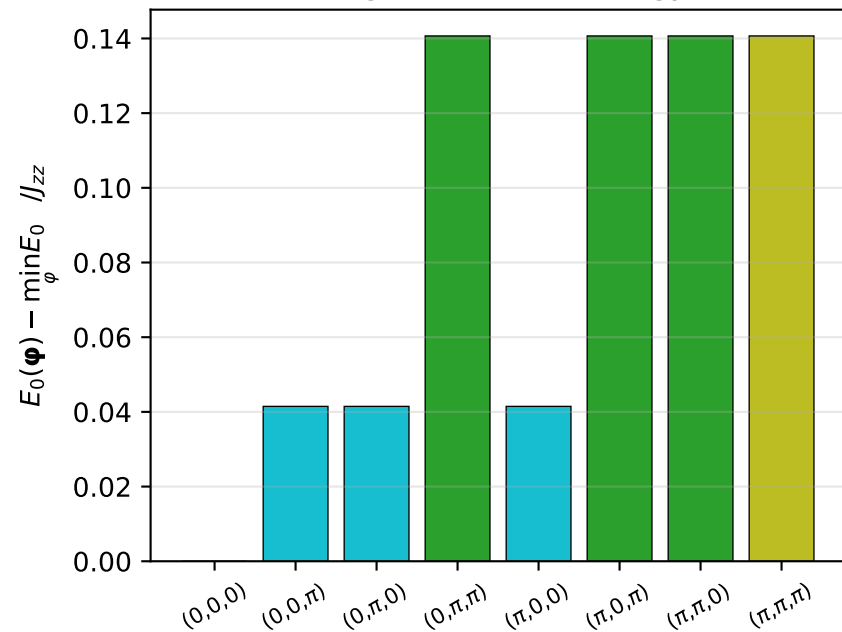
(a) ground-state energy
