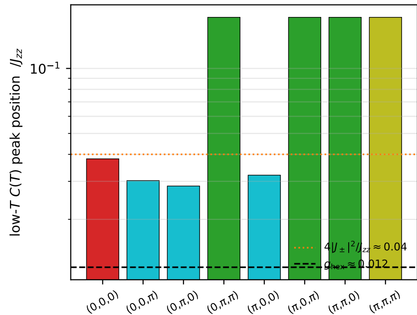
(c) low- T C(T) peak
