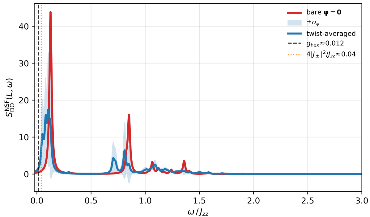
(c) NSF, \mathbf{q} = L = (\pi, \pi, \pi)
