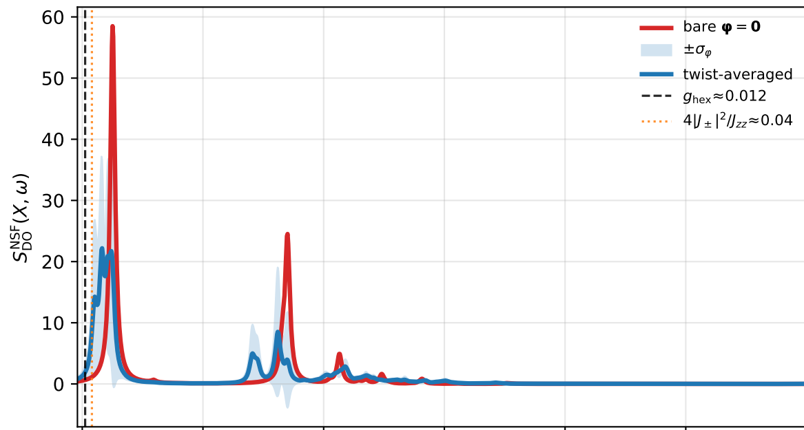
(c) NSF, \mathbf{q} = L = (\pi, \pi, \pi)
