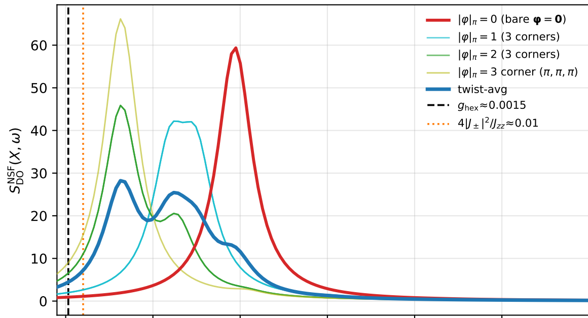
(c) NSF, \mathbf{q} = L , low- \omega zoom
