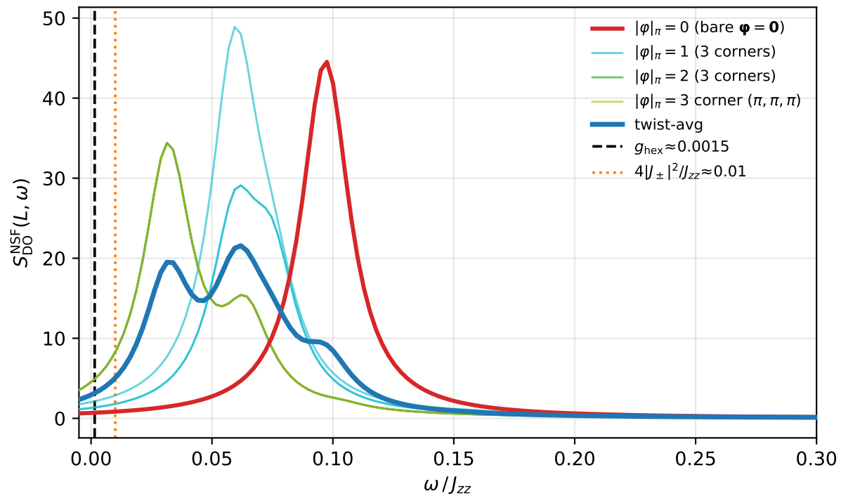
(c) NSF, \mathbf{q} = L , low- \omega zoom
