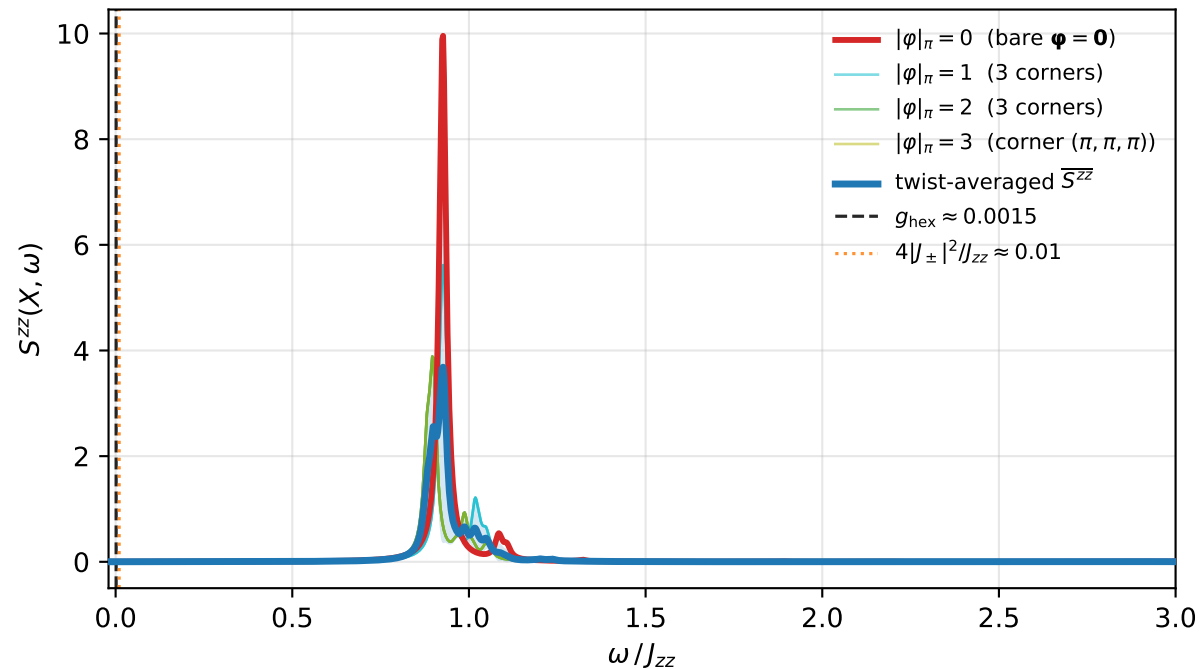
(a) \mathbf{q} = X , per twist corner + average
