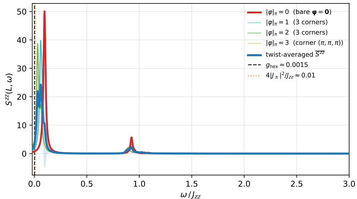
(c) \mathbf{q} = L=(\pi, \pi, \pi) , per twist corner + average
