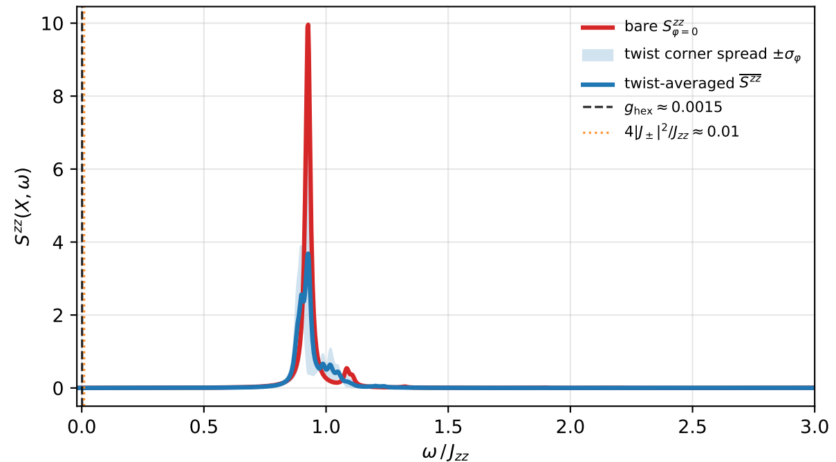
(b) \mathbf{q} = X , bare vs twist-averaged
