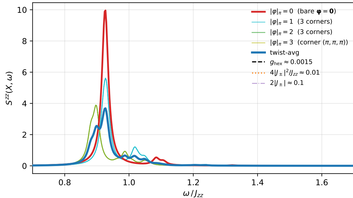
(b) \mathbf{q} = X , spinon-scale zoom
