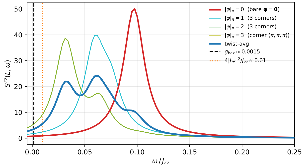
(a) \mathbf{q} = L , low- \omega zoom (photon-relevant scale)
