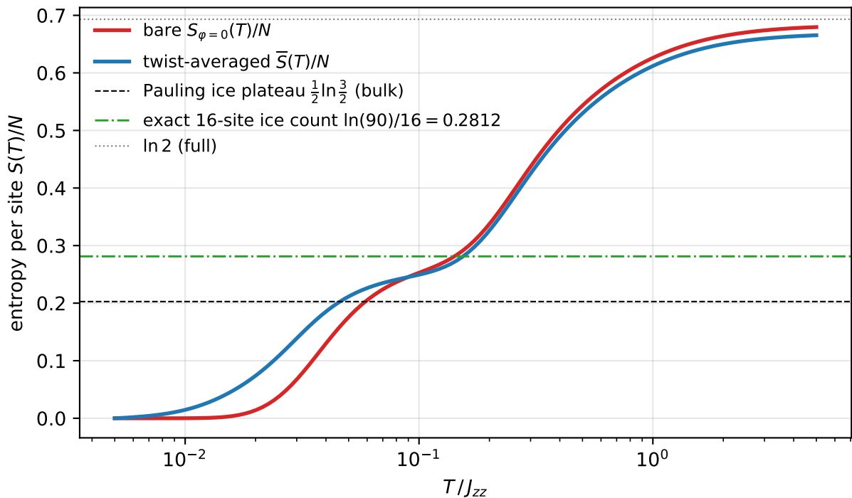
Entropy on the 16-site pyrochlore at J_{\pm} = -0.1J_{zz} : bare vs twist-averaged
