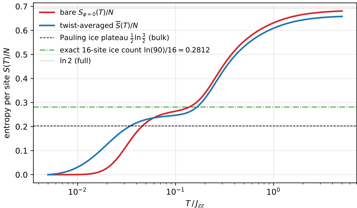
Entropy on the 16-site pyrochlore at J_{\pm} = +0.05J_{zz} : bare vs twist-averaged
