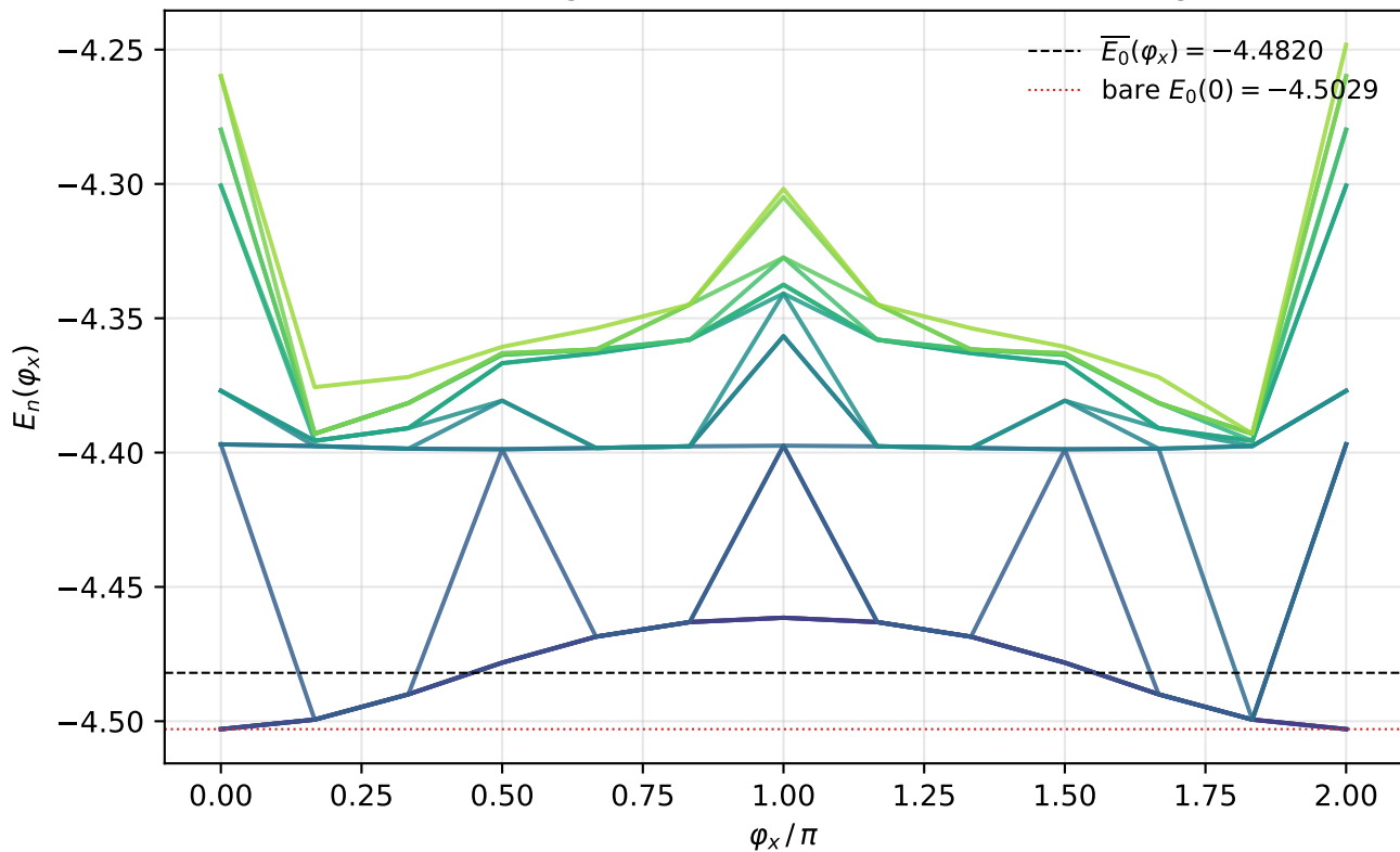
Lowest 16 eigenvalues vs continuous twist along x
